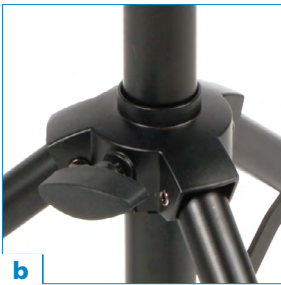
a. Details of height adjustment collar with safety pin b. Details of robust and reliable leg joint
