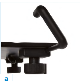
a. Details of LPH/004 laptop clamping device
