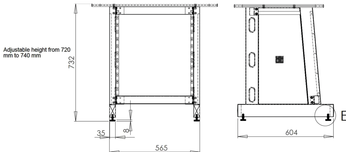
a. View showing a possible configuration of Z/612BK rack stand in combination with Z/460BK project desk system
