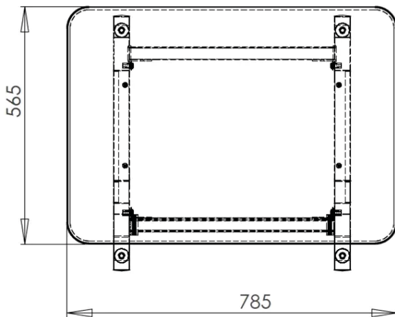
a. View showing a possible configuration of Z/612CY rack stand in combination with Z/630CY project desk system
